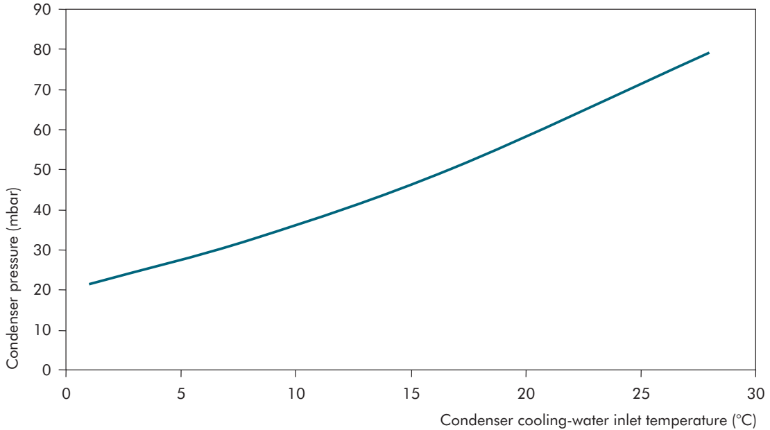
Figure 2.4: Example of the impact of cooling-water temperature on condenser pressure for constant unit load
